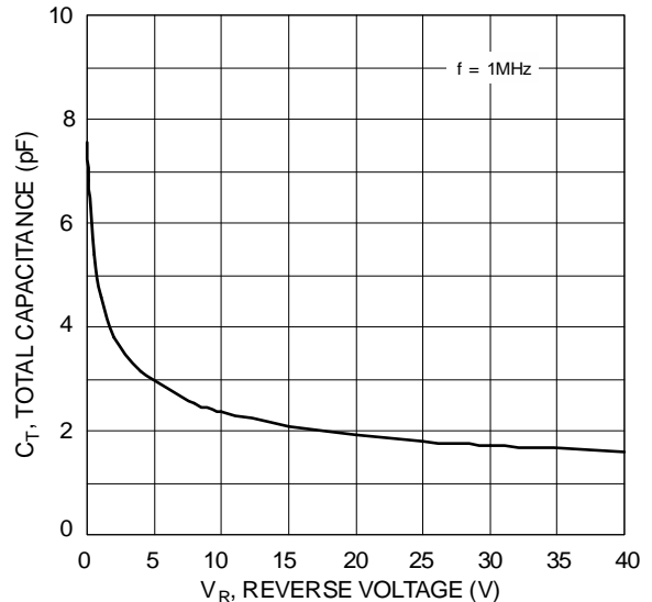
Figure 4 Total Capacitance
